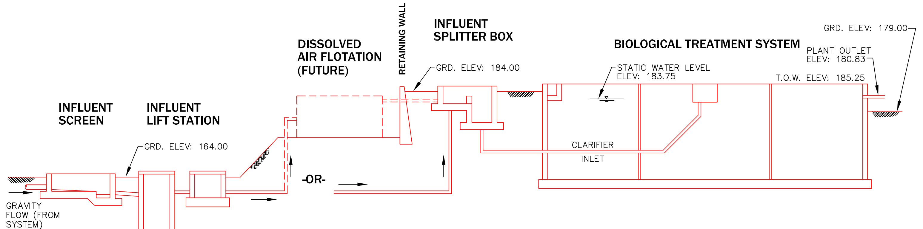
FIGURE 4-02 PROPOSED WWTP UPGRADES - HYDRAULIC GRADE LINE DESIGN DEVELOPMENT REPORT FOR THE LYONS, GEORGIA NORTH WWTP UPGRADE AND EXPANSION FROM 0.670 MGD EXTENDED AERATION TO 1.5 MGD BIOLOGICAL NUTRIENT REMOVAL HOFSTADTER AND ASSOCIATES, INC. CIVIL/ENVIRONMENTAL/TRANSPORTATION CONSULTING ENGINEERS
